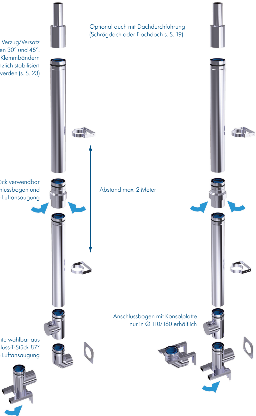
Abb. System Ø 60/100 + 80/125
